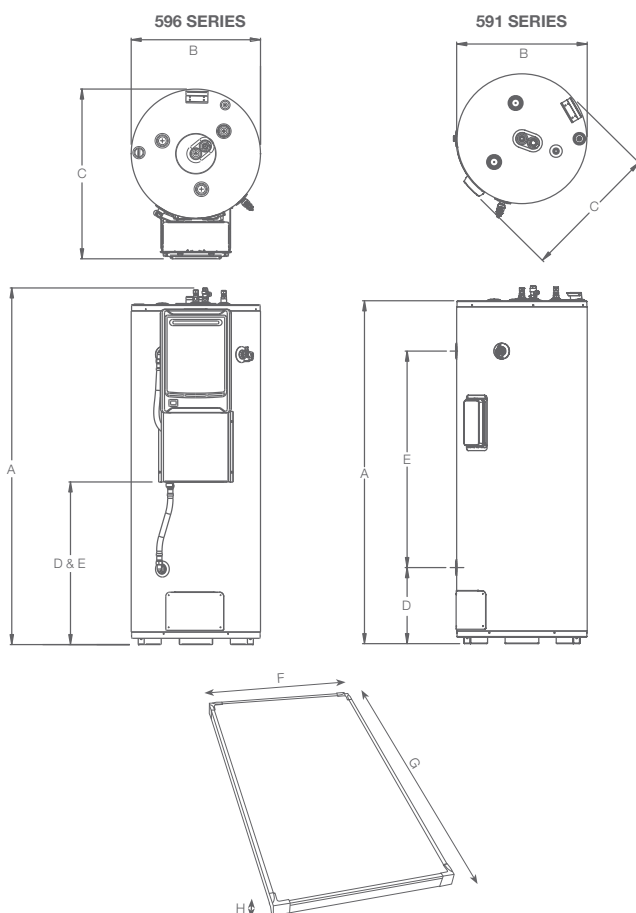
SOLAR COLLECTOR MODELS Dimensions and Specifications
